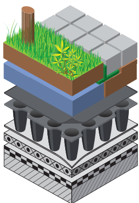
Composition Nophadrain Extensive and Intensive Green Roof System
