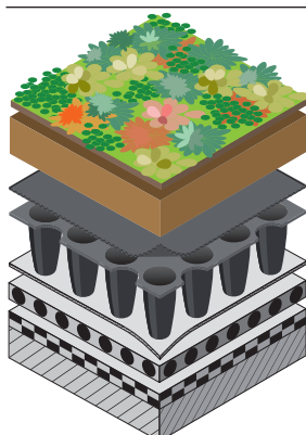
ND 5+1 Drainage System
